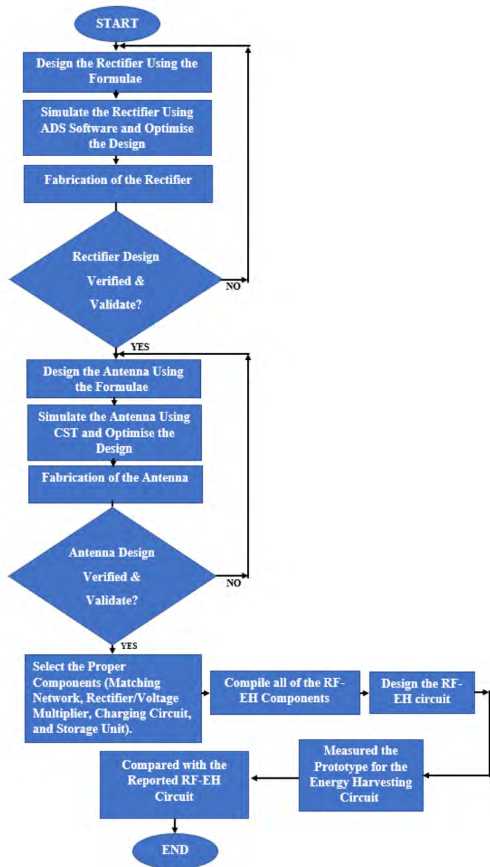
Figure 6. Methodology steps to design the radio frequency energy harvesting circuit.
