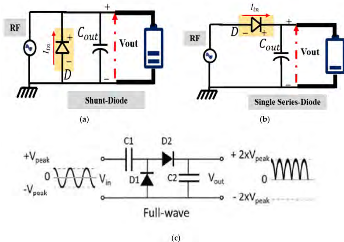
Figure 3. Half-wave rectifier with (a) shunt configuration and (b) series configuration [140], and (c) full-wave rectifier configuration [16].
