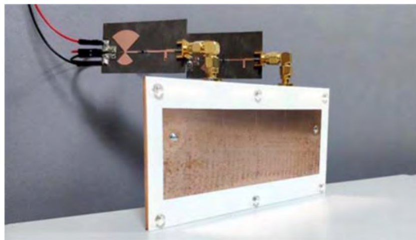
Figure 7. Photographs of the fabricated Rectenna [183].
