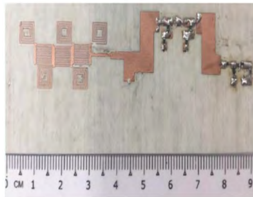
Figure 8. Fabricated prototype of the suggested rectenna [184].
