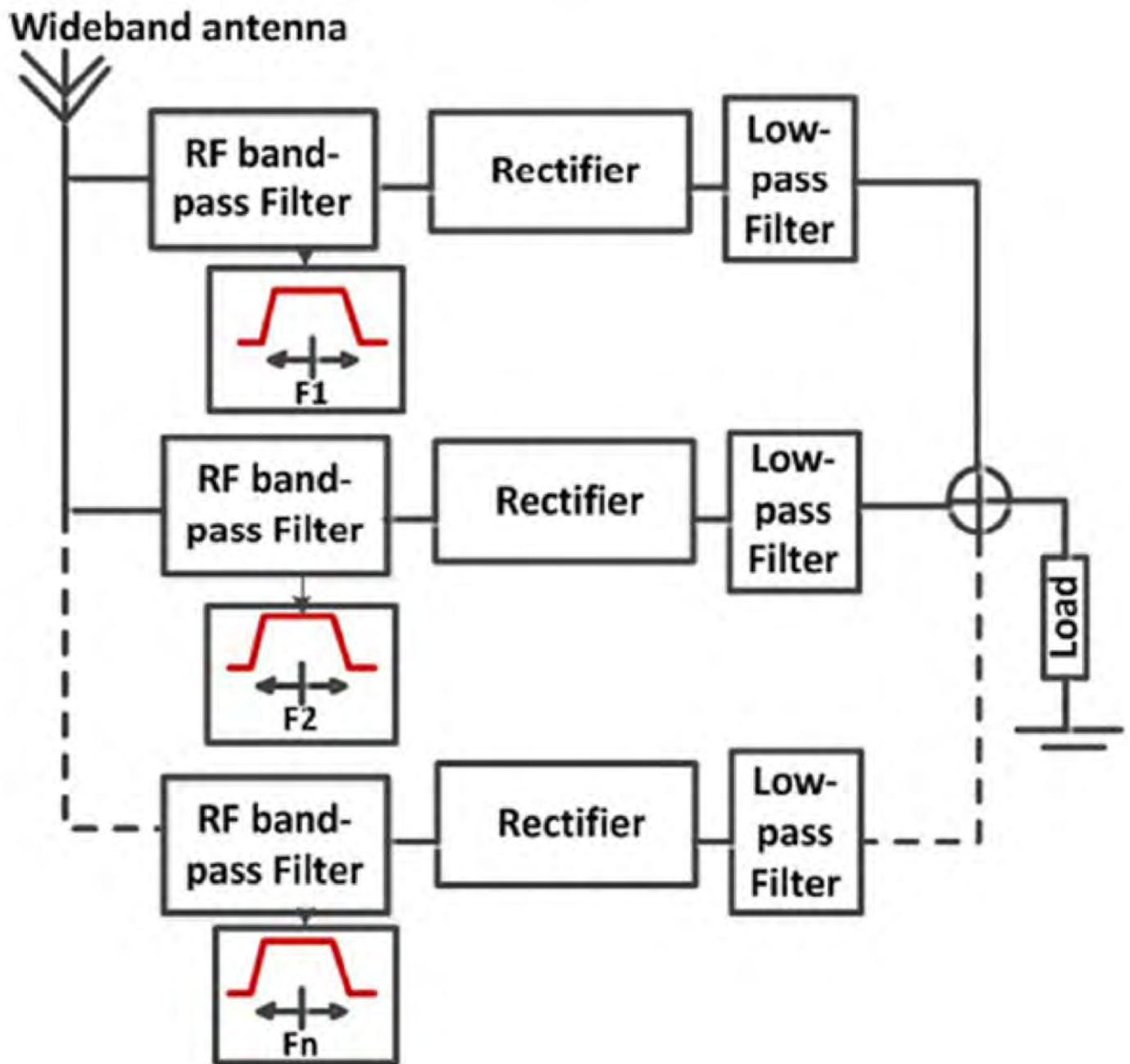
Figure 5. The schematic diagram of the architecture of the multiple RF circuits [169].
