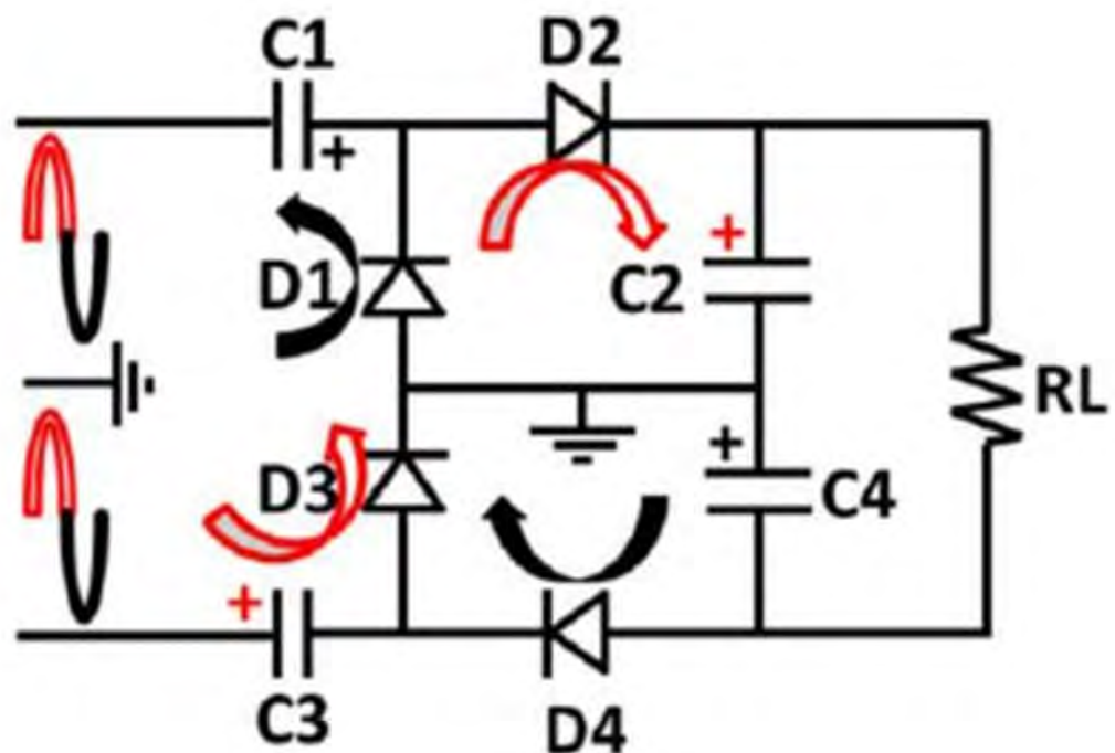
Figure 4. Greinacher rectifier configuration [144].
