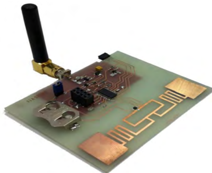
Figure 9. RAMSES Prototype [190].
